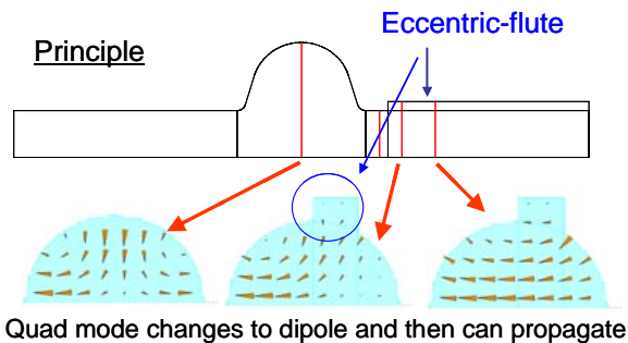
Fig. 13: Basic idea of the eccentric flute
