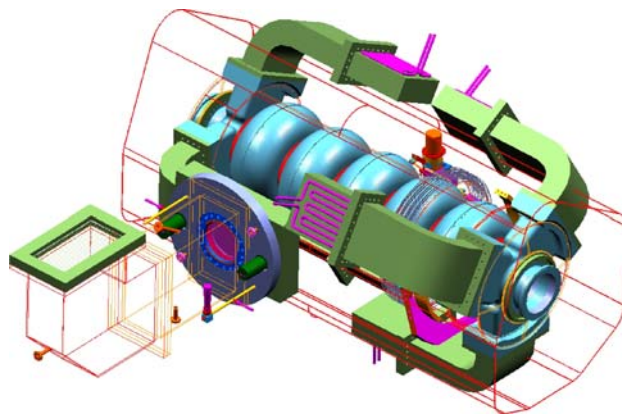
Fig. 2: The JLab ampere-class cryomodule.
