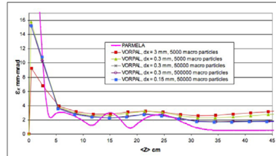
Figure 5: The transverse rms emittance from VORPAL is higher close to the exit of the gun compared to the PARMELA result. The emittance from VORPAL decreases when decreasing the longitudinal cell size but at the end of the gun it still remains approximately three times larger than in PARMELA.
