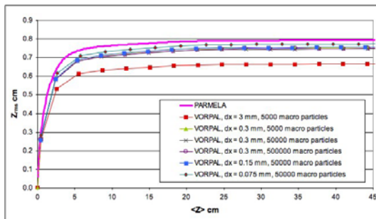
Figure 4: The longitudinal rms size of beams in the VORPAL simulations are shorter than in PARMELA. However, when reducing the longitudinal cell size in VORPAL, the rms size approaches the values from PARMELA.
