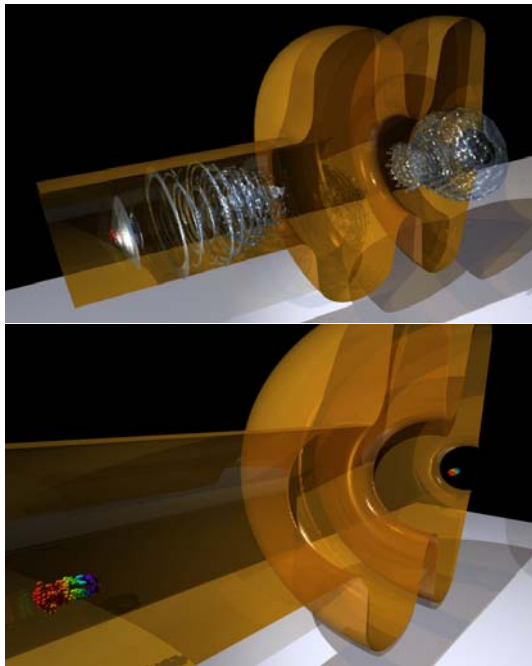
Figure 1: The top image shows a visualization of half of the 1\frac{1}{2} cell electron gun. Electron beams are emitted from a domain on the right side of the gun and propagate to the left. The beam shown in this image is close to the exit from the gun. Isosurfaces of the wakefields that develop are shown as well. The bottom image displays two particle beams from the multi bunch simulations. The beam on the left side is close to exiting the gun while the beam on the right is close to the emitting surface. The color coding of the particles, easier to see in the front beam, show their speed from highest (red) to lowest (blue).
