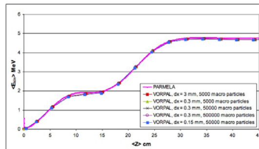
Figure 2: The data from VORPAL on average kinetic energy vs average beam position for different simulation resolutions are in good agreement with results from PARMELA. Thus, the current representation of RF fields in VORPAL is sufficiently close to the one in PARMELA for simulating beam particle kinetic energies.
