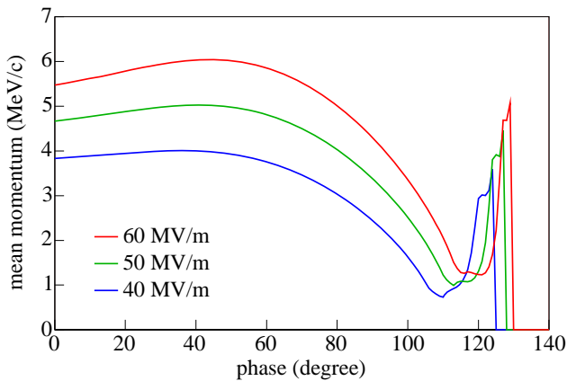
Figure 2: Beam momentum as a function of emission phase. Maximum mean momenta occur at 36^\circ for 40 MV/m, 41^\circ for 50 MV/m, and 44^\circ for 60 MV/m, respectively. Electrons emitted at the phase at which the strongest dark current emission takes place, i.e. 90^\circ , have a significantly lower momentum.
