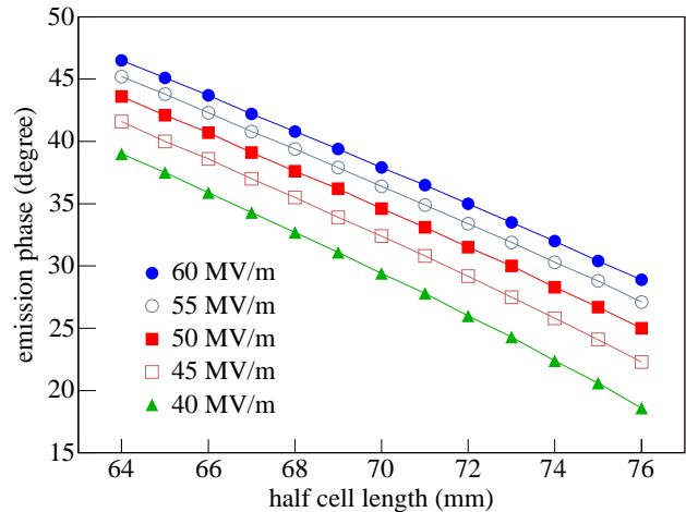
Figure 3: Variation of the optimum emission phase for the highest momentum gain as a function of the half cell length for several RF gradient cases.
