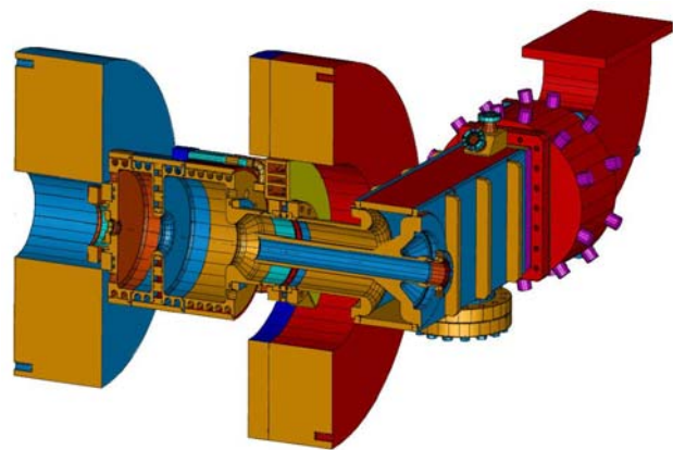
(a) FLASH gun.
