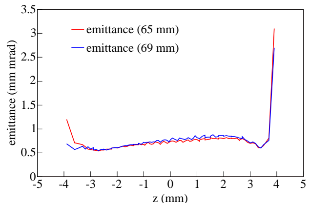
Figure 6: Simulation of the slice emittance for the electron beam with 1 nC bunch charge and a maximum RF field of 50 MV/m. The gun cavities with half cell lengths of 65 mm and 69 mm have been used. The electron bunch is longitudinally divided into 100 slices. Each slice has a charge of 10 pC. At z = 16 m, the emittance is 0.73 and 0.75 mm mrad at the central slices for the cases with a half cell length of 65 mm and 69 mm, respectively.
