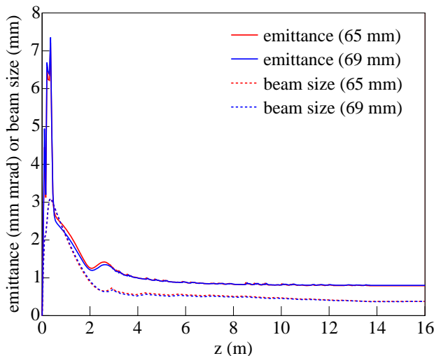
Figure 5: Normalized transverse emittance and beam size evolution for the gun cavities with half cell lengths of 65 mm and 69 mm. The simulations have been made with 1 nC bunch charge. The solenoid field has been configured to be 0.191 T peak field for the 65 mm half cell length case and 0.195 T for the 69 mm case. At z = 16 m, the emittance is 0.79 and 0.80 mm mrad for the cases with a half cell length of 65 mm and 69 mm, respectively. The beam size is 0.38 mm for both cases.
