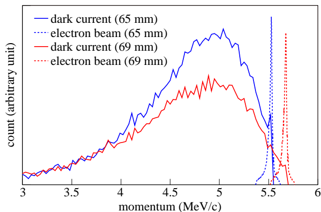
Figure 7: Simulation of the momentum distribution of the dark current and the 1 nC beam at the entrance of the first acceleration module.
