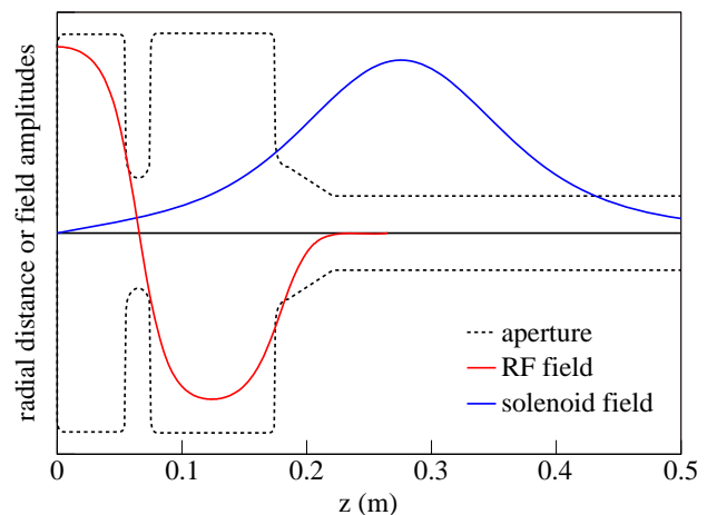
(b) A simplified gun aperture and the field distributions.
