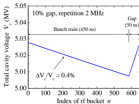
Figure 3: Transient voltage in the injector cavities. Assumed are a total voltage of 5 MV, a beam current of 100 mA, and a 10% bunch-gap at a repetition frequency of 2 MHz.
