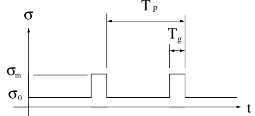
Figure 5: Concept of beam-size modulation.
