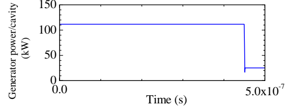
Figure 4: Generator power required for compensating the bunch-gap transient, given in Fig. 3. Per one cavity of the injector. Assumed rf voltage of 1 MV/cavity, a gap ratio of 10%, a gap repetition of 2 MHz, and a beam current of 100 mA.
