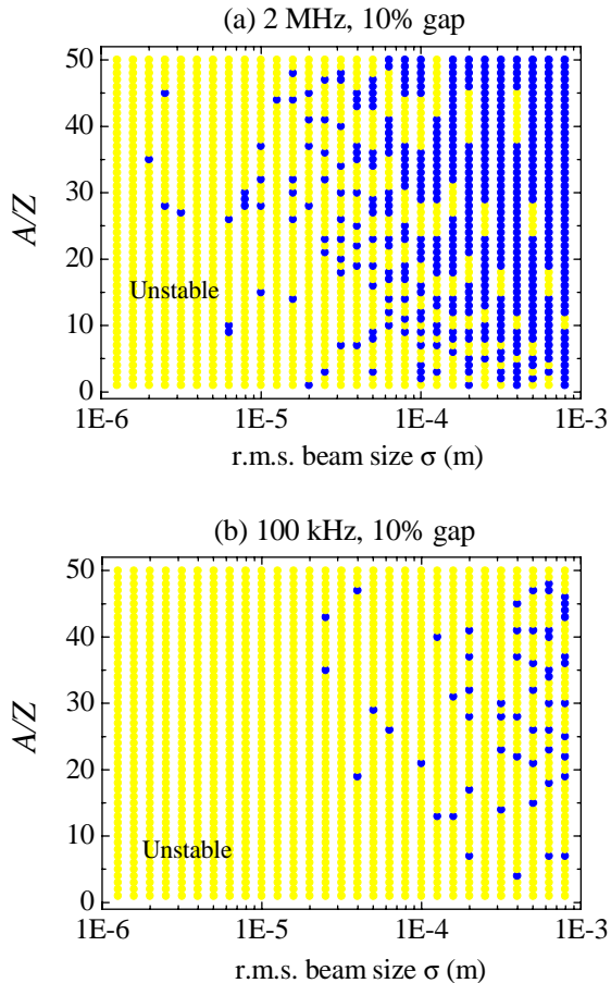
Figure 2: Stability of the ion motions under the bunch gaps. Blue and yellow dots indicate stable and unstable conditions, respectively. Abscissa: beam size (r.m.s.), ordinate: mass number ( A ) per charge number ( Z ) of ions. Assumed 10% ratio of the gap, bunch charges of 77 pC/bunch, and equal beam sizes for the horizontal and the vertical distributions. Repetition frequencies of the gaps are: (a) 2 MHz, and (b) 100 kHz.
