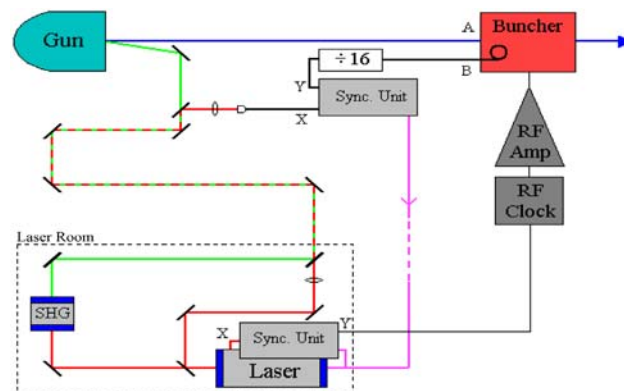
Figure 4: Local and remote synchronisation layouts.
