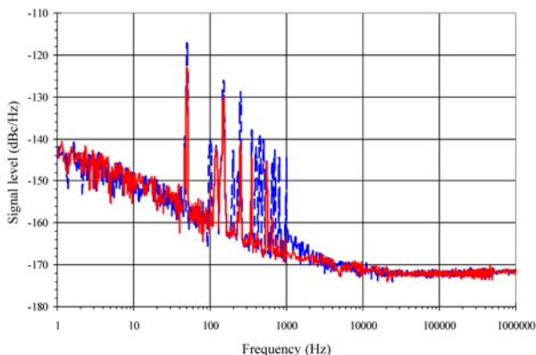
Figure 3: Spectrum showing the noise floor of the HP3047A system with the input mixer powered from the mains (blue trace), or with batteries (red trace).
