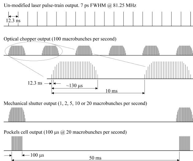
Figure 1: Schematic showing the conversion of the laser oscillator output to the ERLP macrobunch structure.
