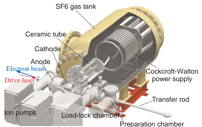
Figure 1: JAEA photocathode electron gun.
