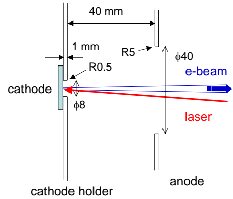
Figure 3: Configuration of gun electrode.
