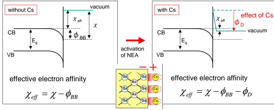
Figure 4: Vacuum potential of GaAs cathode without caesium (left) and with caesium (right). The electron affinity ( \chi ) of bulk GaAs is 4.1 eV and that of bulk \text{Al}_{0.28}\text{Ga}_{0.72}\text{As} = 3.8 eV. The effective electron affinity ( \chi_{\text{eff}} ) of \text{Al}_x\text{Ga}_{1-x}\text{As} is lower than that of GaAs.
