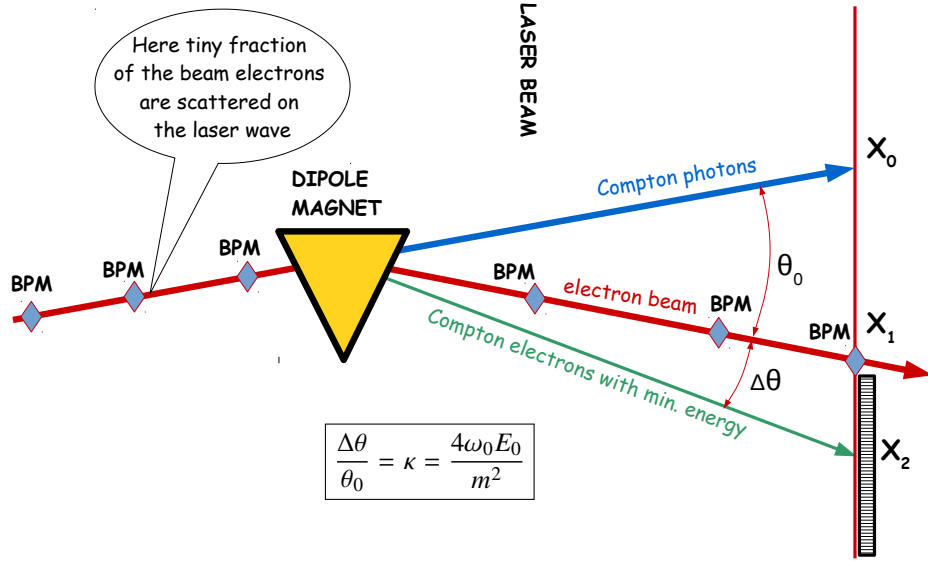
Figure 3: The general layout of ICS experiments.
