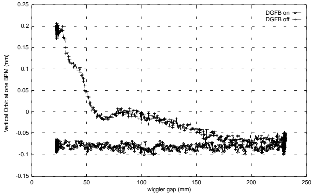
Fig. 2. The orbit change with and without DGFB during wiggler gap change.
