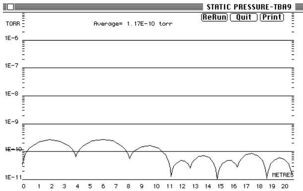
Figure 3 Static pressure profile
