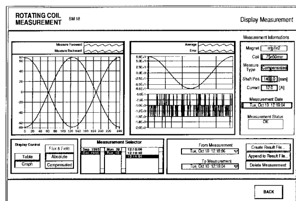
Fig.2. Result display in magnetic measurement program.
