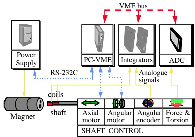
Fig.1. Schematic of the Magnetic Measurement System
