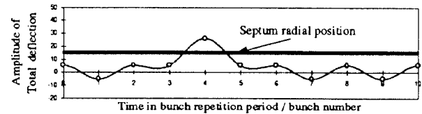
Figure 1-c Total deflection on the different bunches
