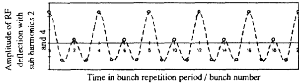
Figure 3-a RF dipole deflection on the different bunches for subharmonic 2 and 4 with 4 bunches in the rise time of the fast kicker
