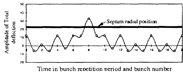
Figure 3-b Total deflection on the different bunches for subharmonic 2 and 4 with 4 bunches in the rise time of the fast kicker
