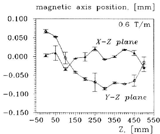
Figure 6: Results on measuring magnetic axis position along the geometrical Z-axis of the quadrupole coil.
