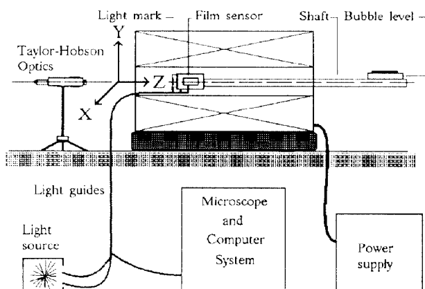
Figure 5: The layout of the experimental facility.
