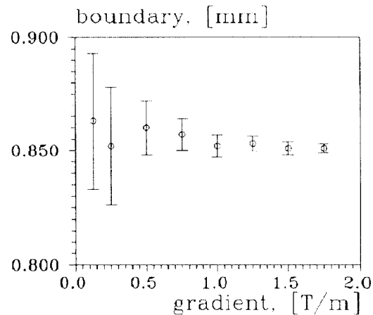
Figure 3: RMS deviation of the boundary position depending on the magnetic field gradient.
