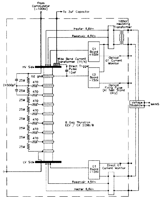
Fig. 2 Crowbar Thyatron
