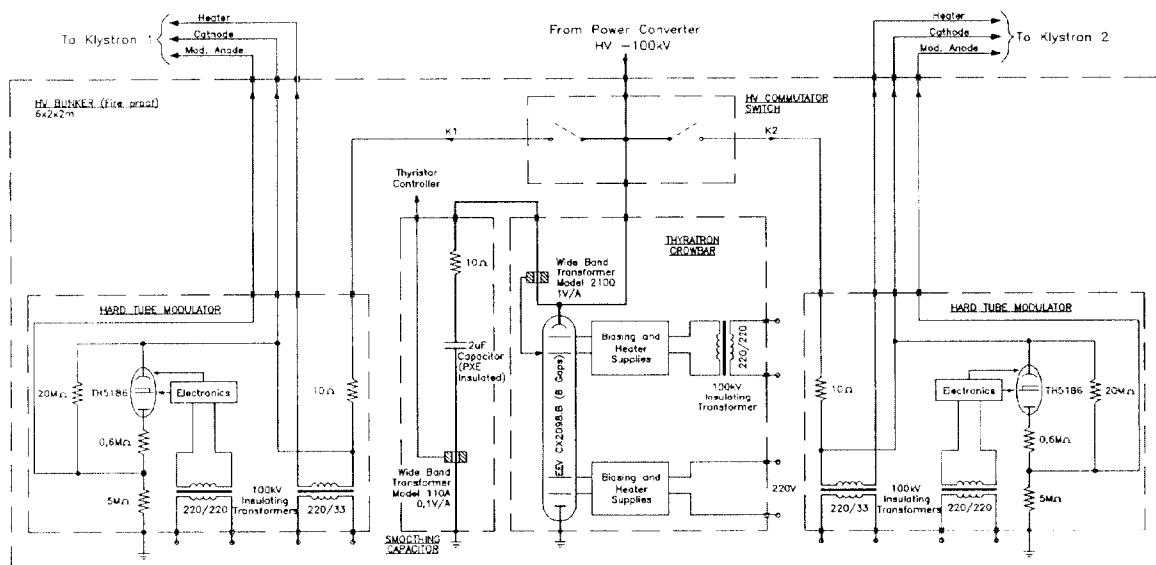
Fig. 1 HV Interface for a LEP2/RF Unit (simplified)
