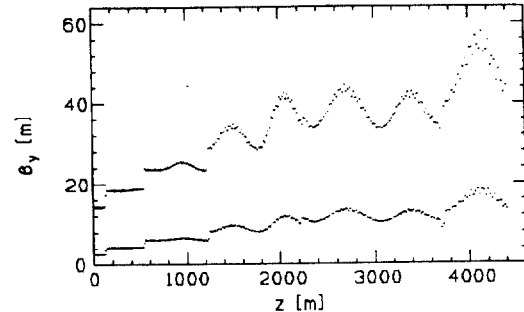
Figure 6. Betatron function in presence of coupling.
