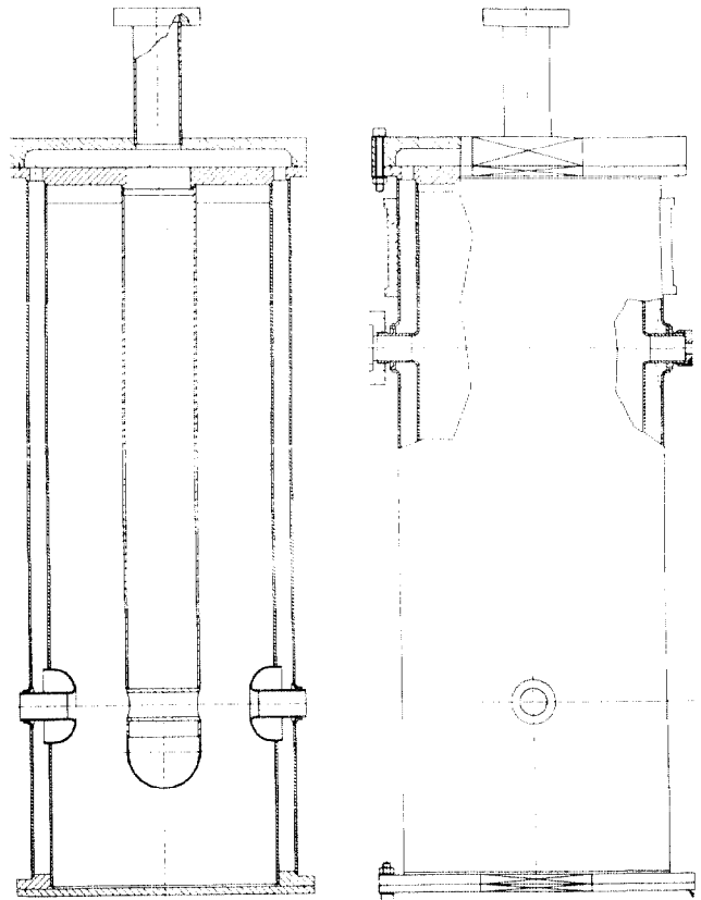
Figure 1. View of the all-niobium quarter wave resonator.
