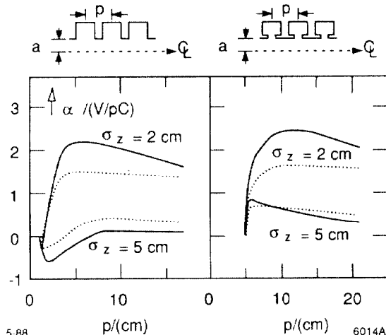
Fig. 1. The parameter \alpha for 2 m of a periodic structure with simple irises (left plot) and one with reentrant irises (right), as a function of structure period p , for bunch lengths of 2 cm and 5 cm. The cavity geometry is sketched at the top. Results are given for iris radius a = 3.5 cm (the solid lines) and for a = 5.0 cm (the dots).
