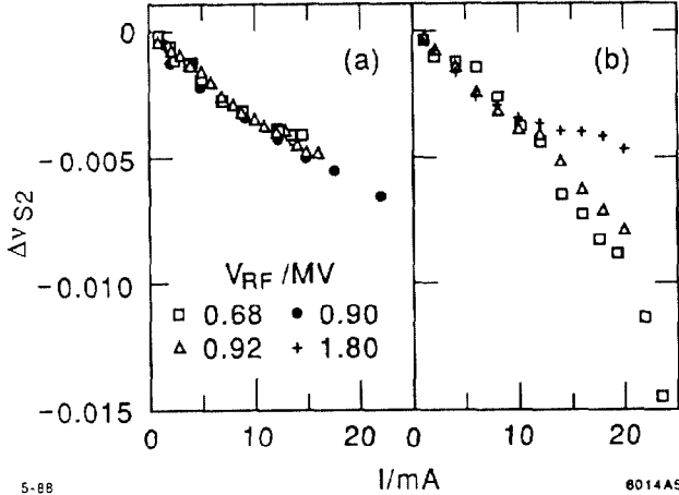
Fig. 6. Shift in the frequency of the quadrupole mode \Delta\nu_{s2} = \nu_{s2} - 2\nu_{s1} . a) New SPEAR II. b) New SPEAR II including the capacitor.
