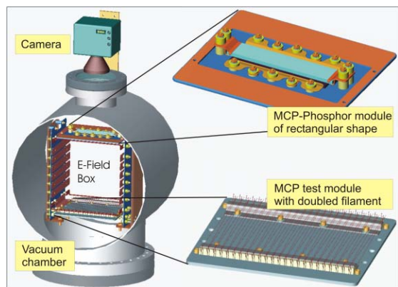
Figure 3: Sketch of the IPM of clearance 175 \times 175 \text{ mm}^2 .
