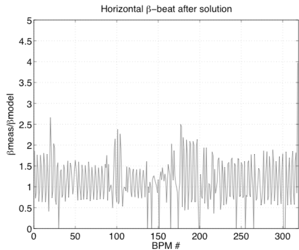
Figure 6: LER horizontal beta-beat, after dialing in closed orbit bump solution.
