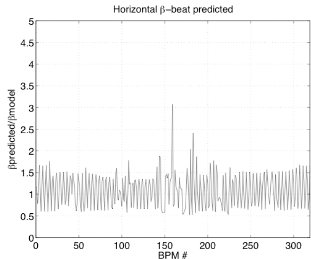
Figure 3: LER horizontal beta-beat, MAD-derived modelled solution.
