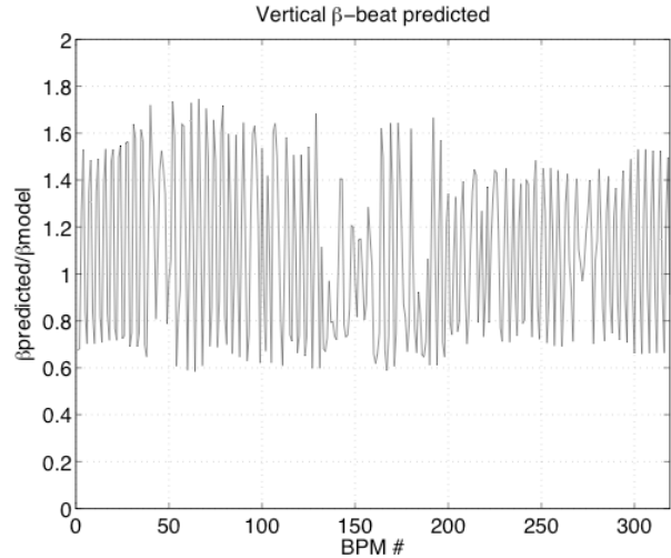
Figure 5: LER vertical beta-beat, MAD-derived modelled solution.
