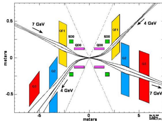
Figure 6: Plan view of a possible IR layout.
