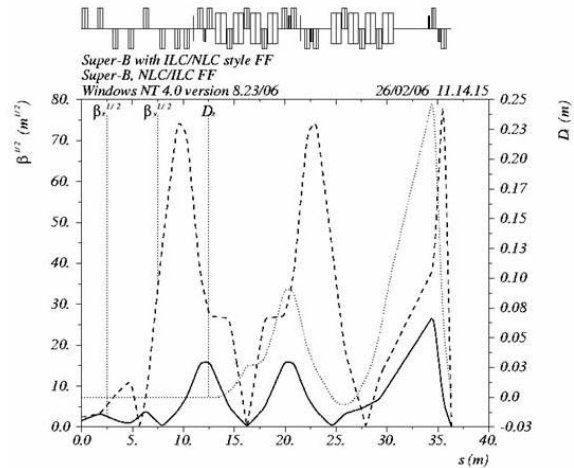
Figure 5: Optical functions in half Final Focus region.
