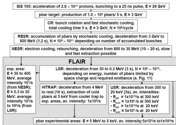
Fig. 3: Estimated antiproton intensities at FLAIR. R_{\text{eff}} is the effective antiproton rate in ring and R_{\text{extr}} the average rate of extracted antiprotons, assuming 90% losses throughout the overall deceleration cycle from the NESR.
