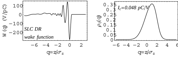
Figure 1: Wake function for the SLC Damping Ring and Haissinski distribution for I_c = 0.048 pC/V.
