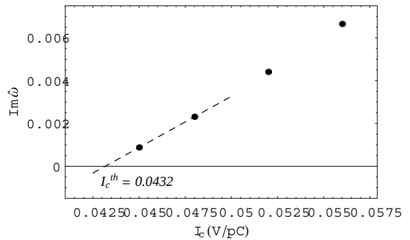
Figure 6: Growth rate \text{Im } \hat{\omega} of unstable mode as function of current parameter I_c .
