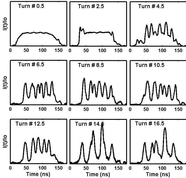
Figure 4: Longitudinal bunch profile measured by the fast Faraday Cup. E_b=20 keV, I_{peak}=23.5 \mu A .
