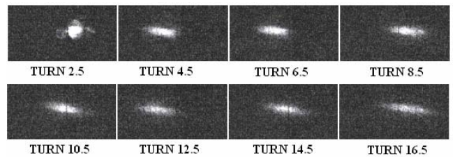
Figure 3: Beam spot produced by the extracted H_2^+ beam on the phosphor screen situated above the median plane. The peak beam current was approx 20 \mu A , beam energy 20 keV, and a pulse length 1 \mu sec . Each frame is approximately 60 mm by 30 mm.
