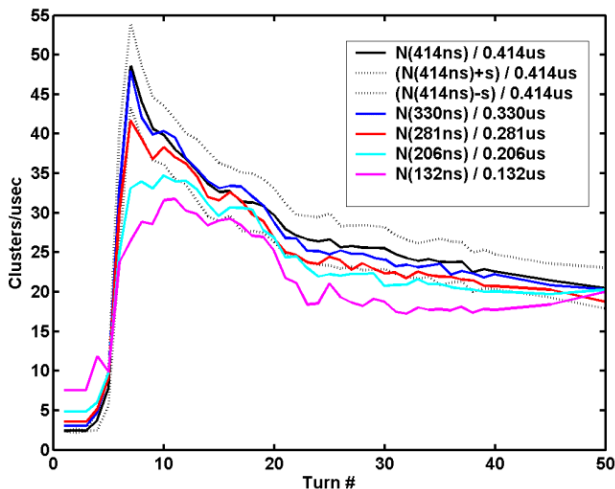
Figure 5: Longitudinal density of clusters vs. turn # for different bunch lengths.
