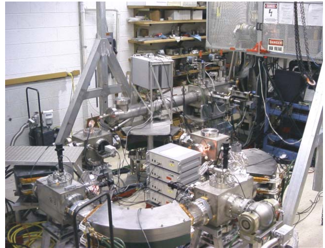
Figure 1: Picture of SIR (11/02/03).
