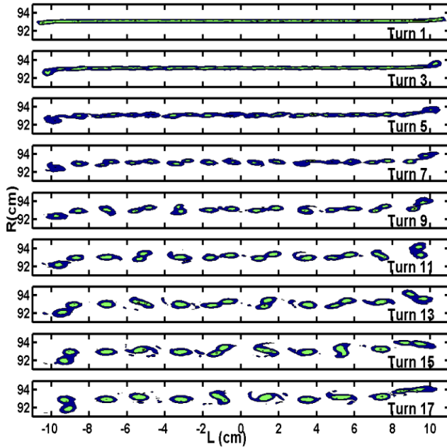
Figure 2: Top view of a 20 keV H_2^+ bunch extracted after a variable number of turns. Peak current is 7 \mu A and length is 22cm. Simulation performed with CYCO.
