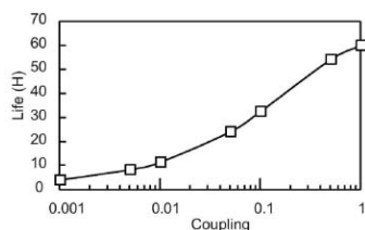
Figure 5: Touschek Lifetime
