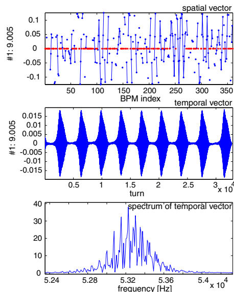
Figure 1: The first betatron mode of a bursting beam. From the top are the spatial vector, temporal vector, and Fourier spectrum of the temporal vector. Red dots are bad BPMs.
