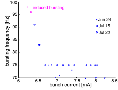
Figure 5: Dependence of bursting period on bunch current.
