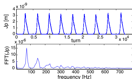
Figure 2: History of the action variable (bursting envelope).
