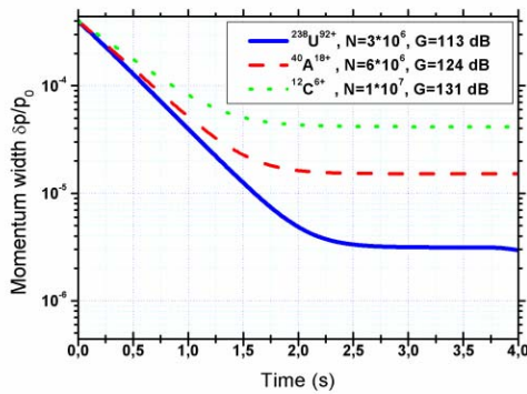
Figure 1. Evolution of the momentum width for different ion species.
