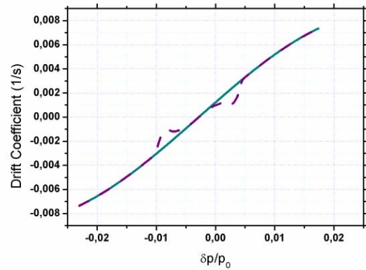
Figure 7. Calculated drift coefficient with signal suppression (dashed) and without (solid).
