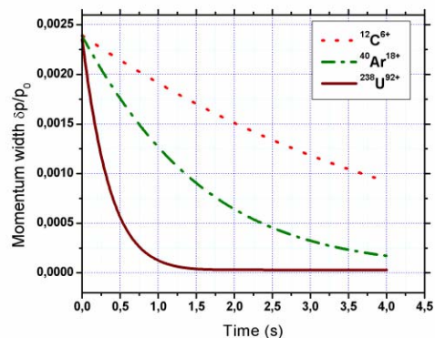
Figure 3. Evolution of the momentum width for different ion species at the CR.
