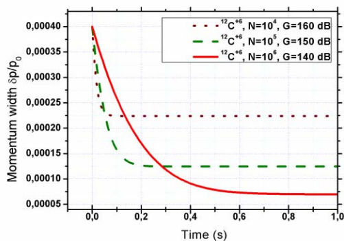
Figure 2. Evolution of the momentum width as a function of time for different numbers of carbon ions.
