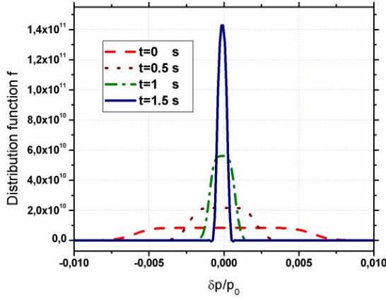
Figure 4. Evolution of the longitudinal distribution function of antiprotons at the CR.
