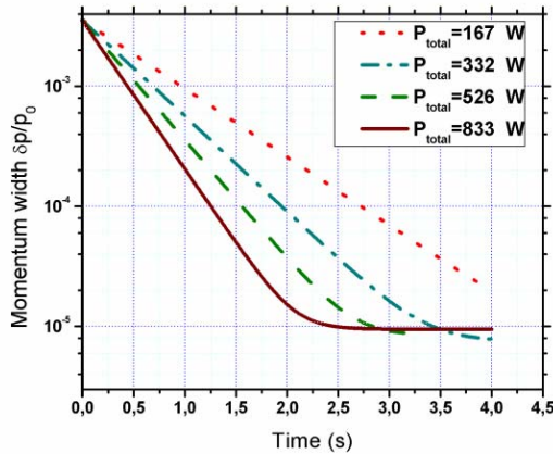
Figure 5. Evolution of the momentum width for a beam of 10^8 antiprotons at the CR for different electrical power.
