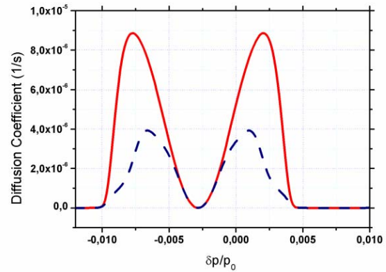
Figure 6. Calculated diffusion coefficient with signal suppression (dashed) and without (solid).
