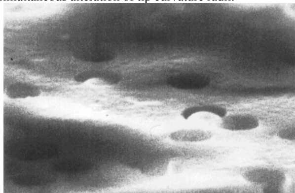
Figure 1: SEM photographs of channels in the nuclear lavsan membrane filled by liquid gallium
