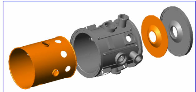
Figure 5: The different layers of the vacuum tank and end flange
