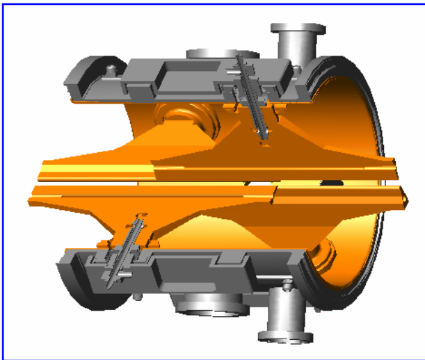
Figure 4: The regular cell of the RFQ.
