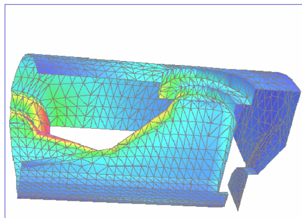
Figure 2: Finite elements model of the end cell in "OPERA - 3D" code
