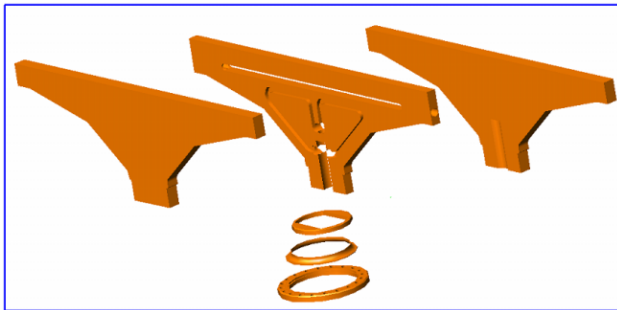
Figure 7: The parts of the vane
