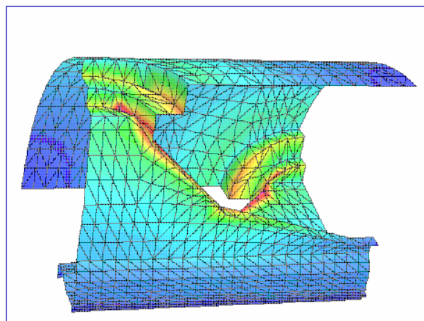
Figure 1: Finite elements model of the regular cell in "OPERA - 3D" code
