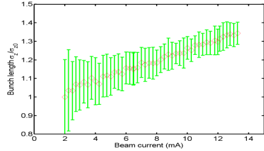
Figure 1: Single-bunch beam bunch length versus bunch current.
