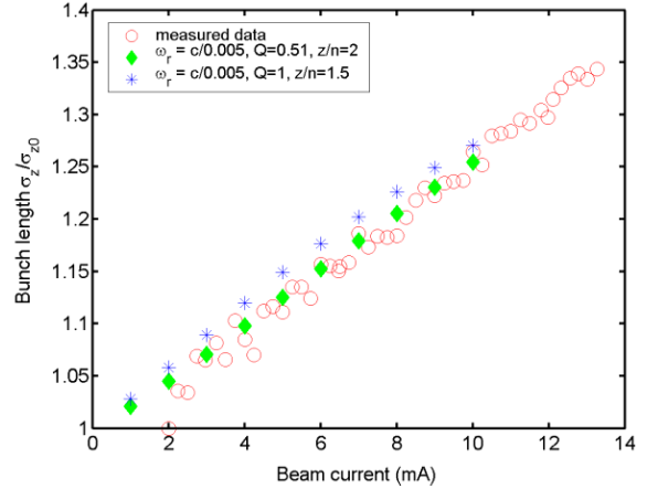
Figure 6: The bunch length measurement data compare with two impedance with the same \omega_r = c / 0.005 and Q=0.51 , Z/n = 2 \Omega or Q=1 , Z/n = 1.5 \Omega .
