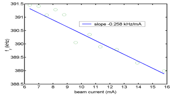
Figure 2: Single-bunch beam vertical betatron frequency shift with beam current. Circles are measurement data and solid line is a linear fit with slope of -0.258 kHz/mA.
