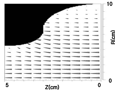
Figure 3: The cell geometry for the third harmonic rf cavity and fundamental mode electric field.
