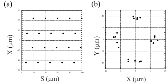
Figure 6: Example of the crystal structure. 6(a) is the side view of the horizontal 4-lines crystal at the particle number of 7.8 \times 10^5 . 6(b) is the front view of the single shell at the particle number of 1.6 \times 10^6 .
