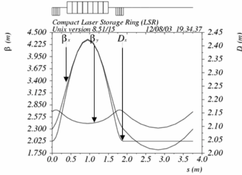
Figure 5: Lattice parameters in one period when the betatron tune is (1.45, 1.44).
