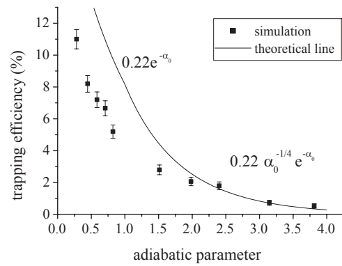
(b) The calculated trapping efficiency with theoretical line
