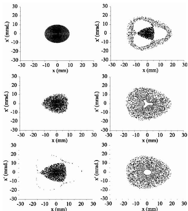
Figure 5 Snapshots of particle distribution during crossing (very slow crossing / \epsilon=1 \times 10^{-10} )
