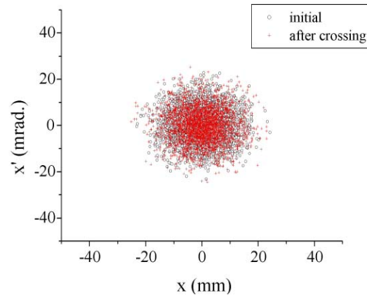
Figure 3 The particle distribution before and after opposite crossing
