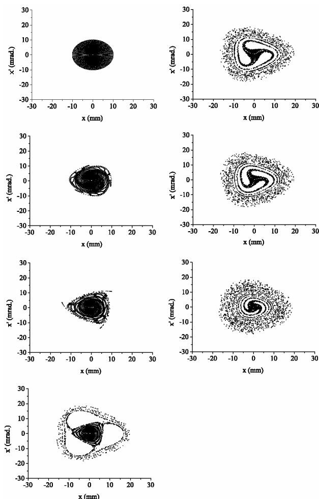
Figure 4 Snapshots of particle distribution during crossing ( \epsilon=2 \times 10^{-7} )
