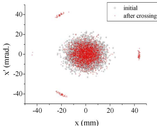
(a) The particle distribution before and after crossing (adiabatic parameter = 1)
