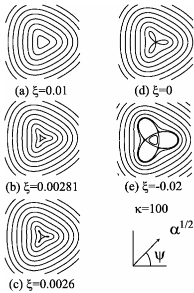
Figure 1 The phase space topology for third integer resonance crossing
