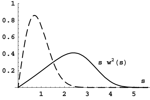
Figure 1: The radial distribution s w^2(s) compared with the distribution in absence of space charge (dashed line) for a strong space-charge strength. All quantities are dimensionless.
