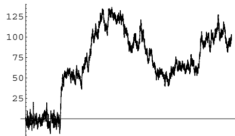
Figure 3: Student process with \nu = 3.0
