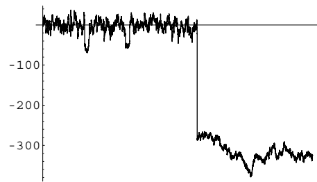
Figure 2: Student process with \nu = 2.0
