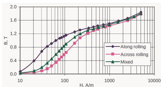
Figure 2. B-H curve anisotropy of M250-50A steel.
