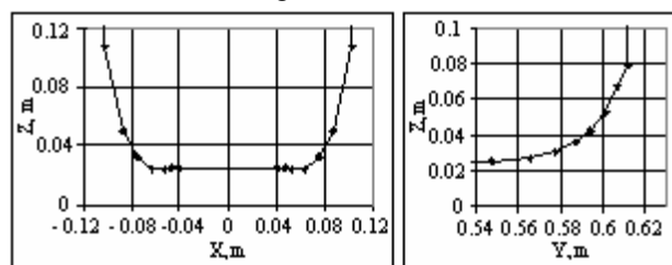
Figure 2: Pole profile and edge chamfers.
