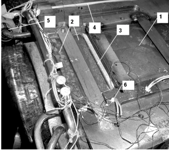
Figure 3: Top view of PDP1s dipole end part with measuring coils: 1 - regular laminated yoke, 2 - the insertion from SMP 1321, 3 - flat coil, sensitive to the longitudinal B_z component, 4 - coil, wound around the bracket, 5 - Rogowski-coil around the cooling tube, 6 - temperature sensors.
