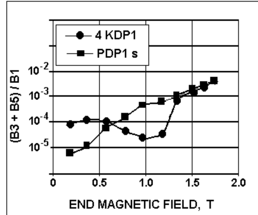
Figure 5: The sum of sextupole and decapole harmonics as function of the main magnetic field.
