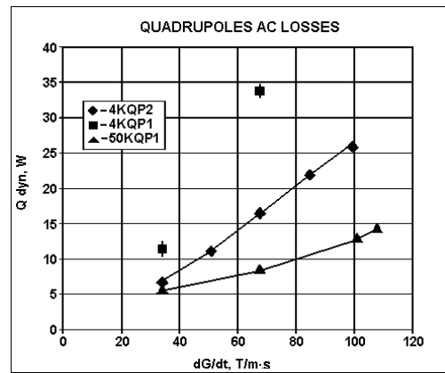
Figure 8: AC losses at 4K in model quadrupoles 50KQP1 and 4KQP2 as function of dG/dt . ( G = 34 \text{ T/m} )
