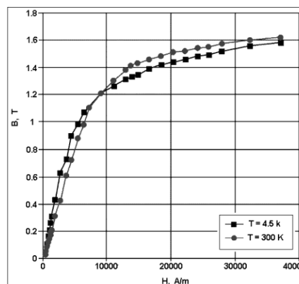
Figure 2: The B-H curves of the Corovac sample.
