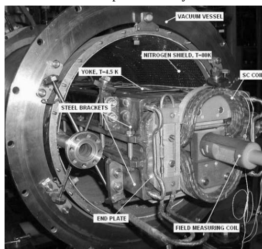
Figure 1: PDP1s dipole inside cryostat.
