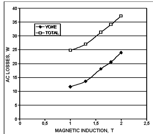
Figure 6: AC power losses in the model 4KDP5.
