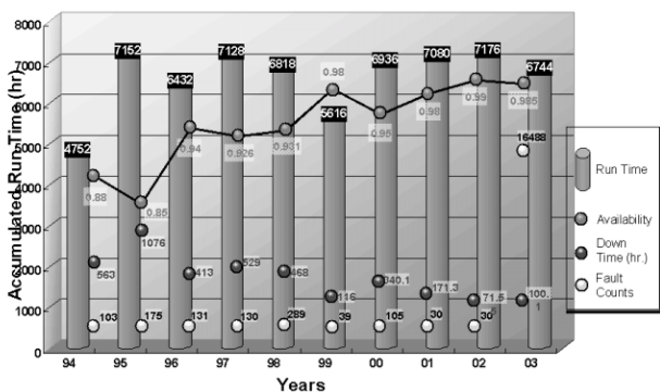
Figure 3. Availability, down time, and fault count of modulator during 1994 to 2003.
