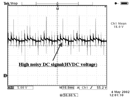
Figure 5. Digital filtering of high noisy DC signal (Continuously sampled and average)
