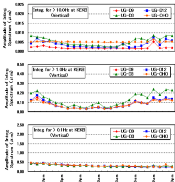
Figure 5: The time serial spectrum densities of KEK.
