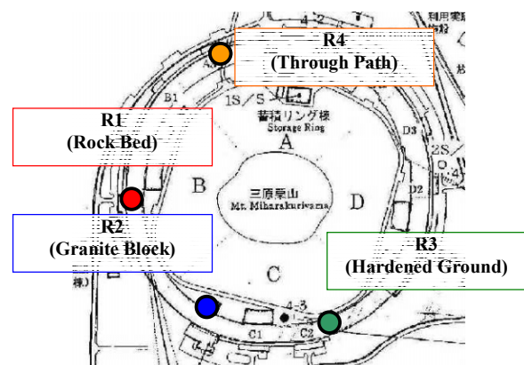
Figure 2: Measurement points in the SPring-8 ring
