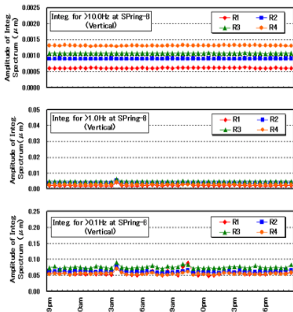
Figure 6: The time serial spectrum densities of SP8.
