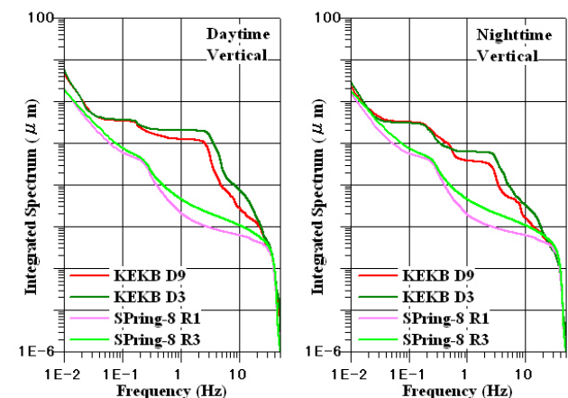
Figure 4: Integrated spectra for vertical GM in the daytime and night-time at KEKB and SPring-8 (Vertical)
