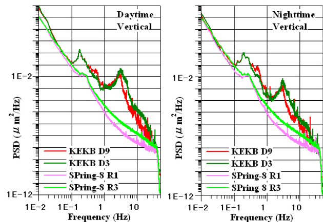
Figure 3: PSDs of vertical ground motion in the daytime and night-time for KEKB and SPring-8.
