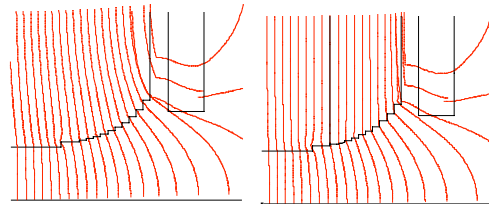
Fig. 14 Flux distributions at the magnet edges of a solid magnet (left) and a laminated magnet (right).
