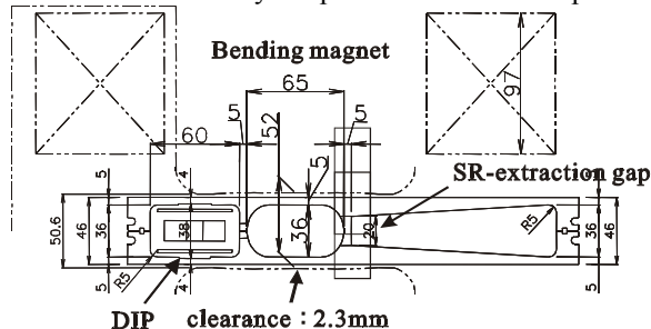
Fig.3. The layout of the cross section of the bend chamber. The DIP is equipped on the side of beam chamber. The inner gap of chamber is open with 20 mm height.
