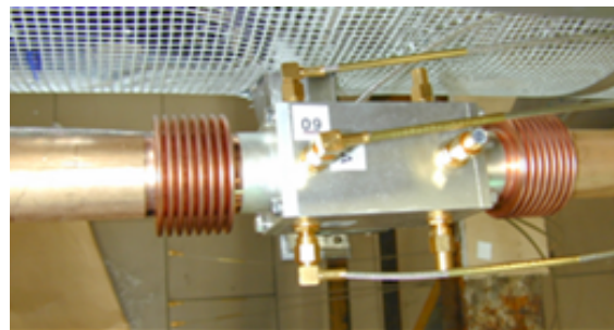
Figure 3: Top view of a WPM sensor.
