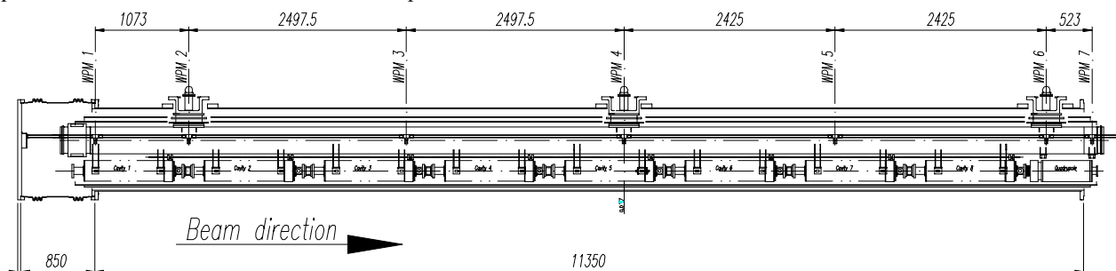
Figure 2: The longitudinal positions of the WPM sensors in cryomodule # 4.
