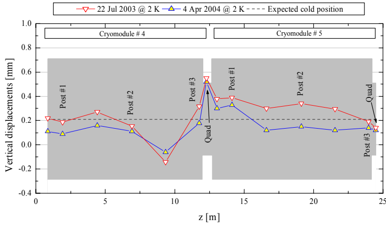
Figure 5: Vertical displacements measured by the WPM system.
