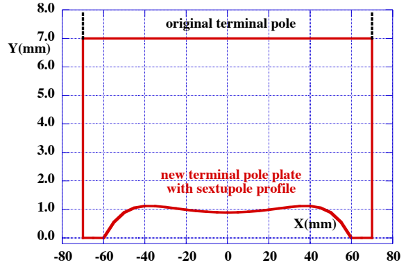
Figure 4: Section of the shaped iron plate glued on the terminal pole (horizontal and vertical sizes not in scale).
