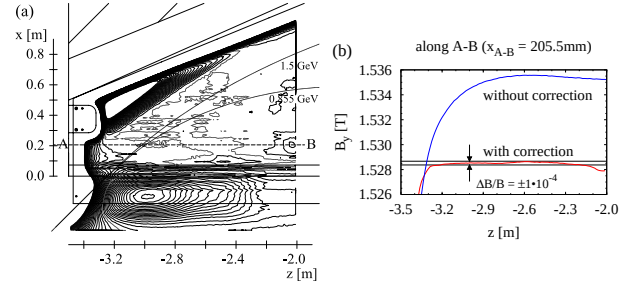
Figure 7: (a) \Delta B_y(x, 0, z) in steps of 0.2 mT with symmetric correction. (b) B_y(x_{A-B}, 0, z) along A-B.
