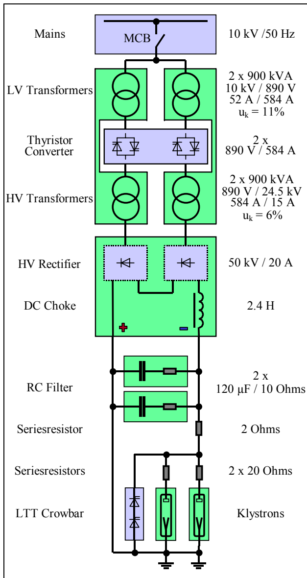
Figure 1: Main circuit diagram DESY-II installation
