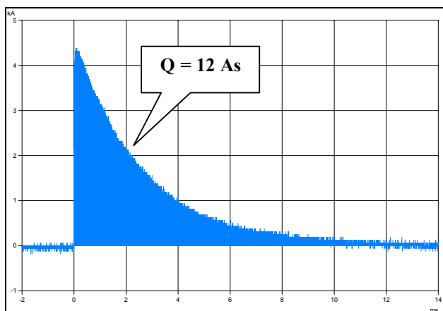
Figure 2: Capacitorcharge DESY-II installation
