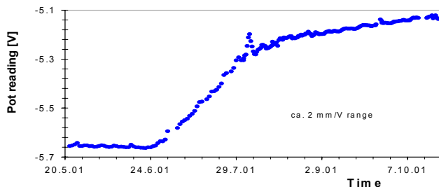
Figure 6: HLS sensor reading from May to Oct. 2001
