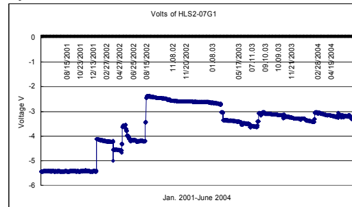
Figure 4: Voltage of the 2 nd HLS sensor of girder 1 in section 7 from Jan. 2001 to June 2004
