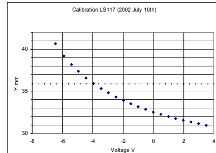
Figure 3: Calibration curvature
