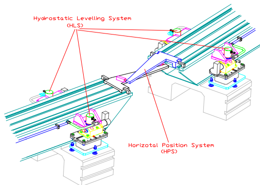
Figure 1: Layout of the HLS
