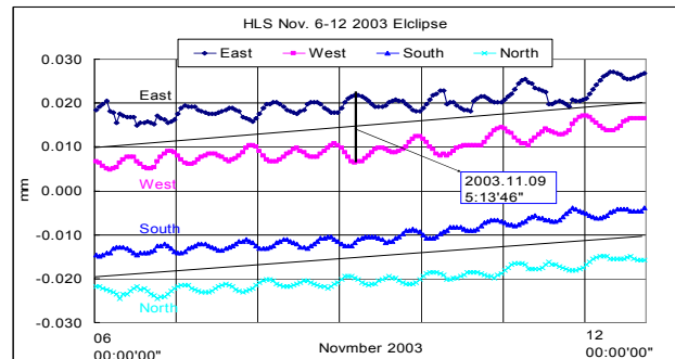
Figure 10: Oscillations of the SLS HLS
