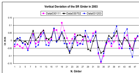
Figure 8: Mean deviations of all girders at the beginning, in the middle and at the end of year 2003.
