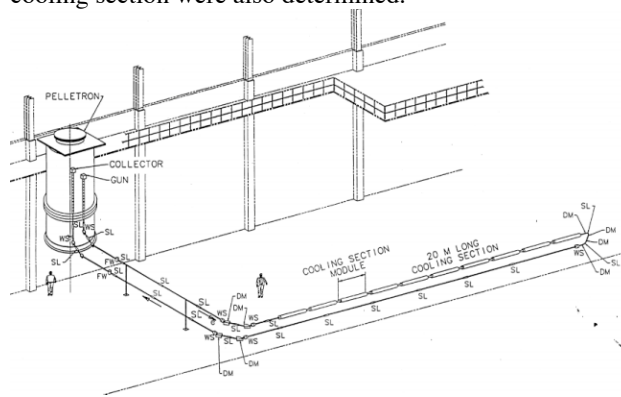
Figure 3: Full Scale Prototype System
