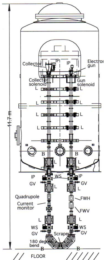
Figure 2: Recirculation Experiment
