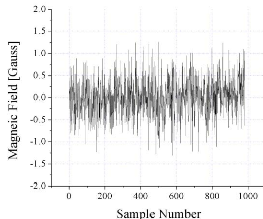
Figure 3: Measured system noise converted to magnetic field.
