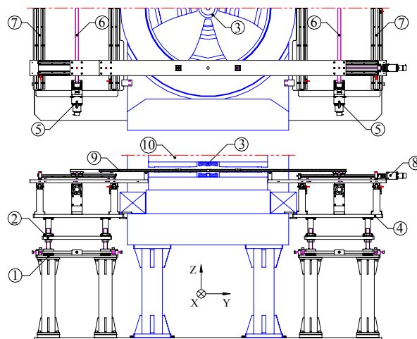
Figure 1: Cyclotron magnet and Hall probe mapping system: alignment stages ① and ②, center plug ③, mapping stage ④, x-axis motors ⑤, x-axis ball screws ⑥, x-axis guide rails ⑦, y-axis motor ⑧, Carrier ⑨, and magnet ⑩.
