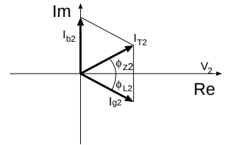
Figure 2: The phasor diagram for the 2nd higher harmonic component.
