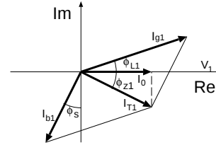
Figure 1: The phasor diagram for the fundamental component.
