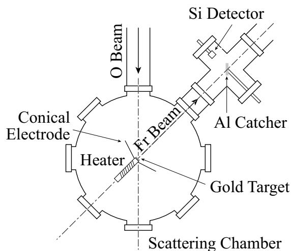
Figure 1: Schematic diagram of the target area.
