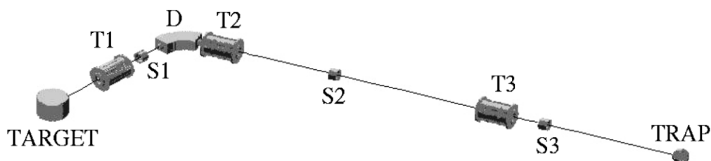
Figure 2: 3-keV francium beam line.
