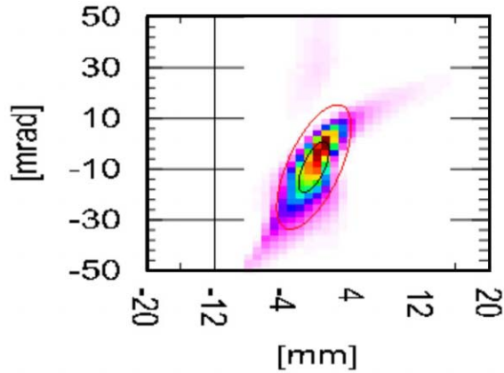
Figure 4 : 1 mAe of O 6+ horizontal emittance beam at 60 KV (0.22 \pi .mm.mrad at 1 \sigma normalized)
