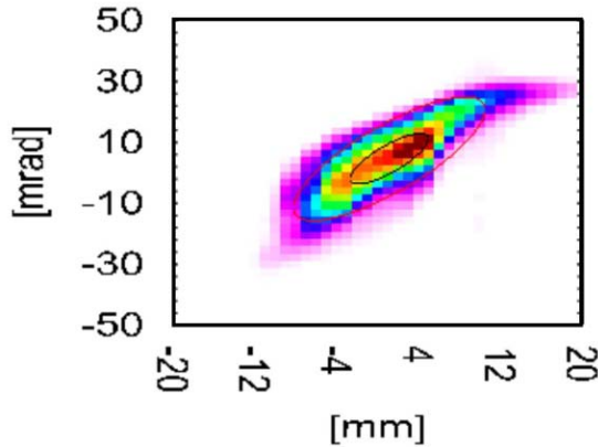
Figure 5 : 1 mAe of O 6+ beam vertical emittance at 60 KV (0.22 \pi .mm.mrad at 1 \sigma normalized)
